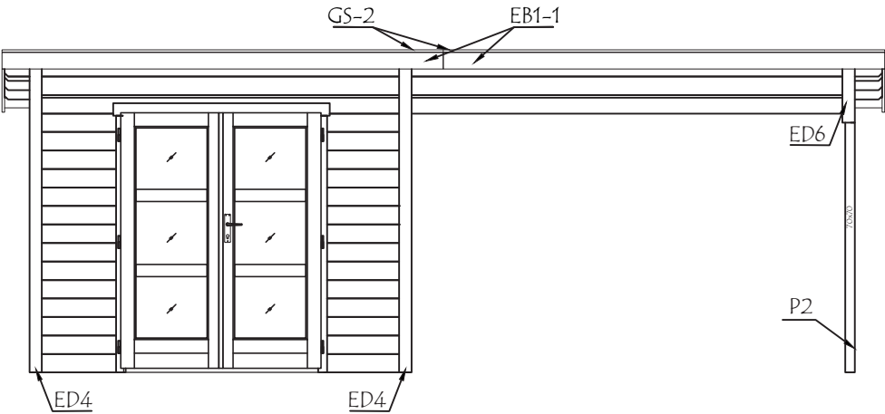
VORDERANSICHT-FRONT VIEW SCALE: NOT TO SCALE
