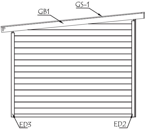
SEITENANSICHT (LINKS) - SIDE VIEW (LEFT) SCALE: NOT TO SCALE
